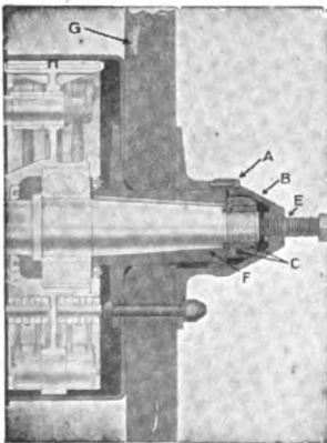
Ready demountability of Sheldon wheel hub. Remove parts A, B, and C, replace B (hub cap), insert E (set screw), and screw against shaft. Tap back of wheel G till it comes loose.
